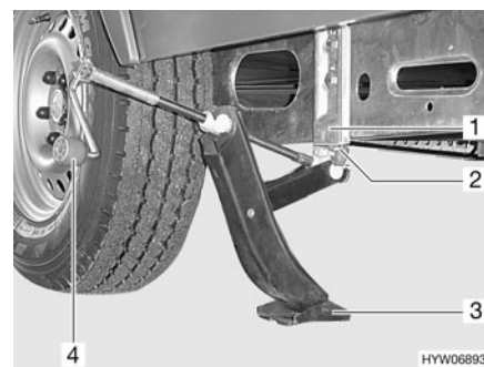
Fig. 196 Cric AL-KO
